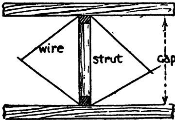
Strut straight. Wires and gap correctly adjusted
